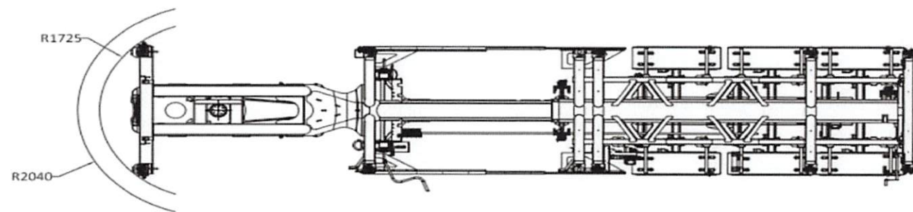
Middle-Rear EXT Container chassis 1 x 20F(rear space)
